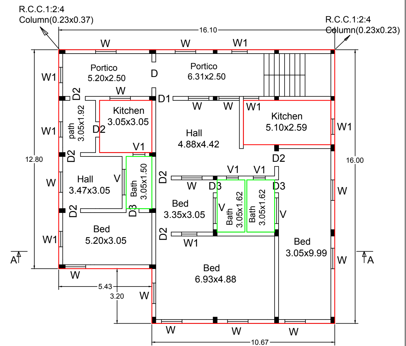
PLAN - First Floor - House
