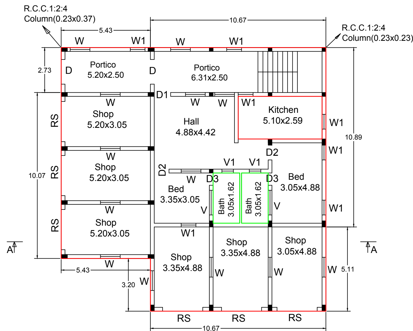
PLAN - Ground Floor (House & Shop)
