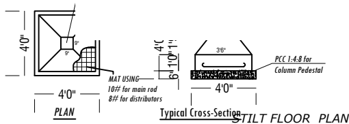
FOOTING DETAILS
