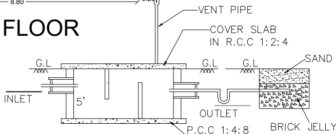
SECTION-AB
