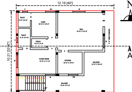
PROPOSED F.F PLAN
