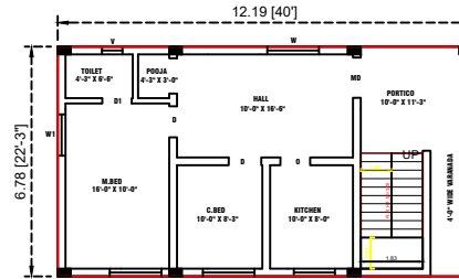
PROPOSED G.F PLAN
