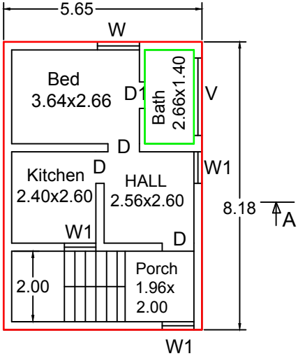
PLAN - First Floor
