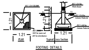
FOOTING DETAILS
