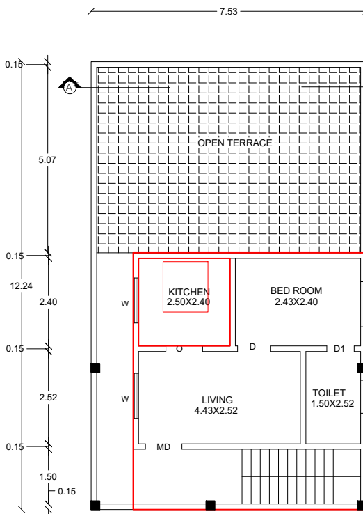
SECOND FLOOR
