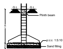
FOUNDATION DETAILS
