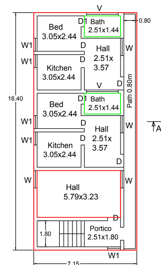
PLAN - First Floor
