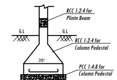
Typical Cross-Section FOOTING DETAILS
