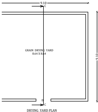
DRYING YARD PLAN
