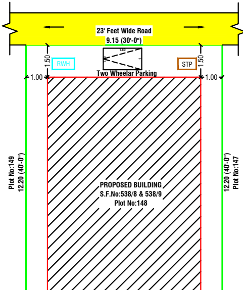
SITE PLAN SCALE 1:100 & As Per Document
