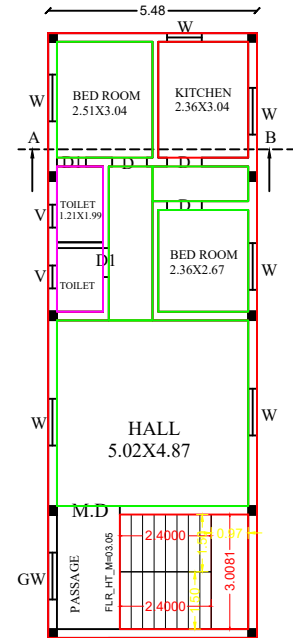
PRO.SECOND FLOOR
