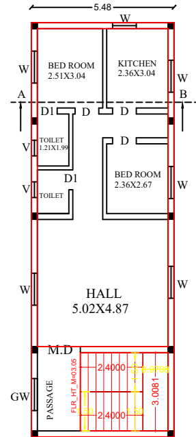
EX.FIRST FLOOR
