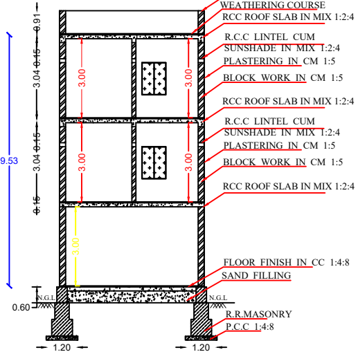
SECTION ON-'AB'
