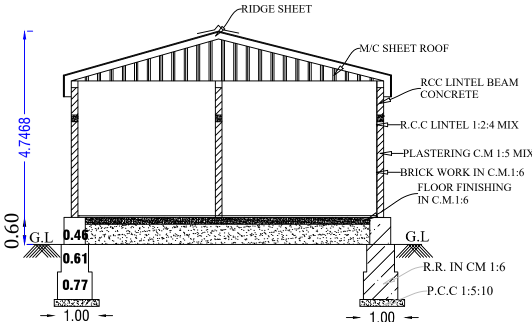
SECTION ON-"AB"
