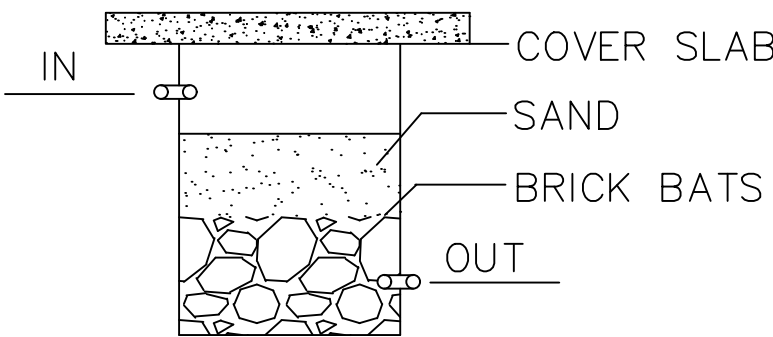
SECTION
