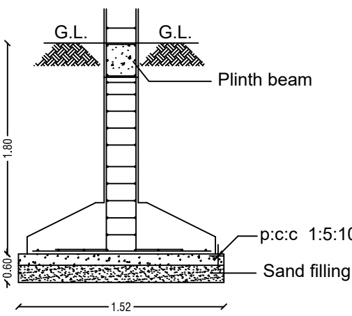
FOUNDATION DETAILS
