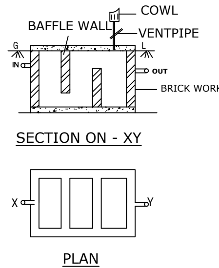
SEPTICTANK DETAILS
