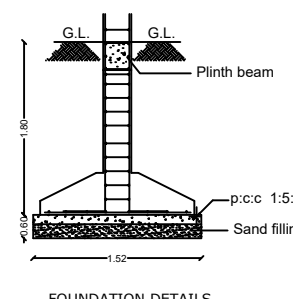
FOUNDATION DETAILS
