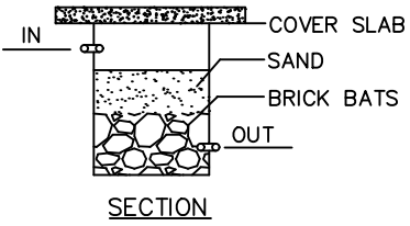
RAINWATER HARVEST
