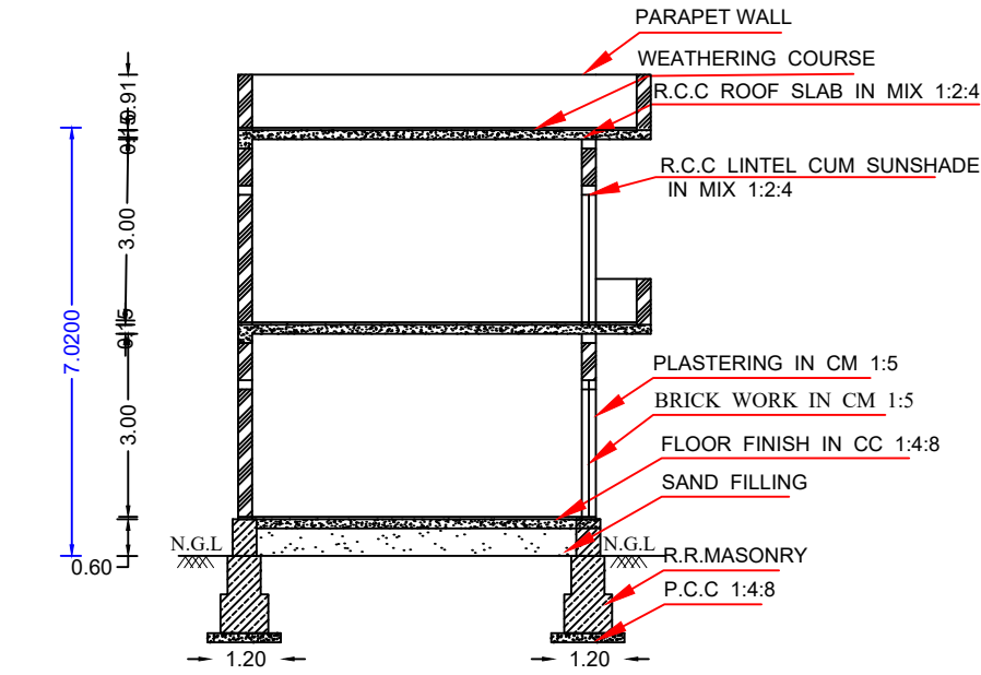
SECTION ON-"AB"
