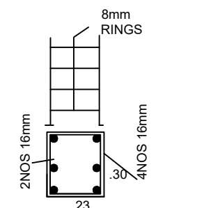
COLUMN DETAILS
