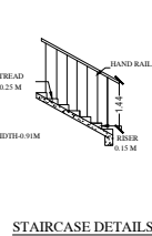
STAIRCASE DETAILS
