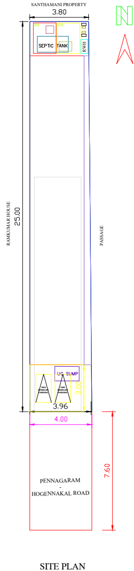
SITE PLAN
