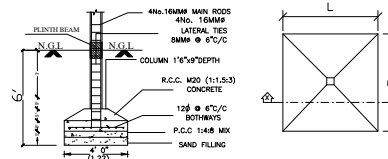
SECTION (X-X)
