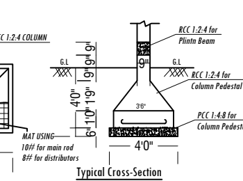
FOOTING DETAILS
