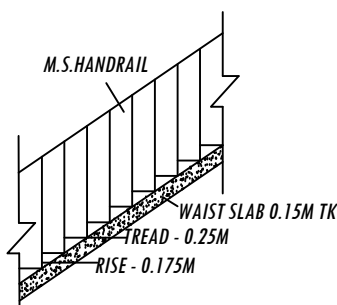
STAIR CASE DETAILS
