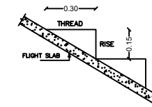
STAIRCASE DETAILS
