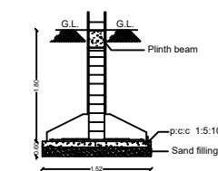
FOUNDATION DETAIL
