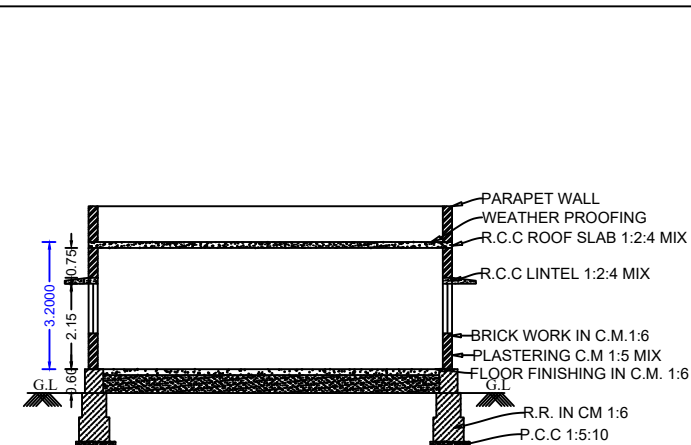
SECTION ON-"AB"
