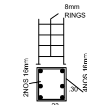
COLUMN DETAILS
