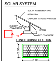
SOLAR SYSTEM
