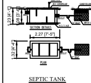
SEPTIC TANK
