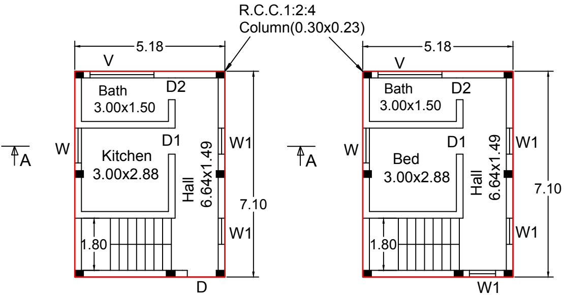
PLAN - Ground Floor
