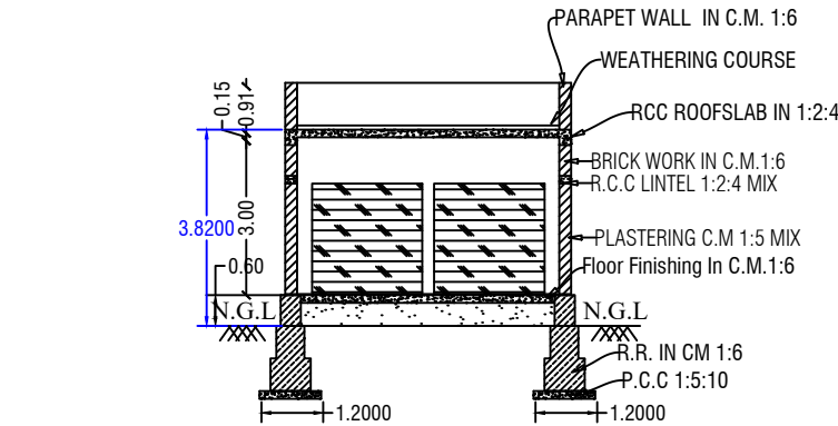
SECTION ON-AB
