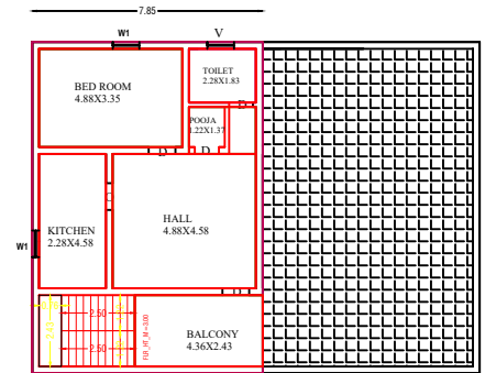
PROPOSED SECOND FLOOR PLAN
