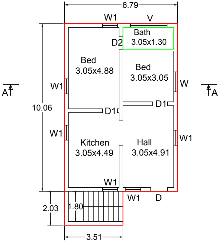
PLAN
