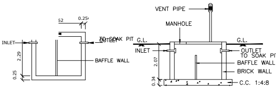
PLAN SEPTIC TANK
