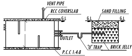
SECTION DETAILS NO DISPERSION TRENCH DETAILS
