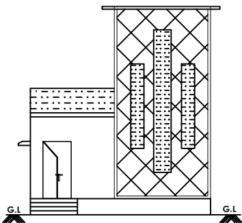
ELEVATION PLAN
