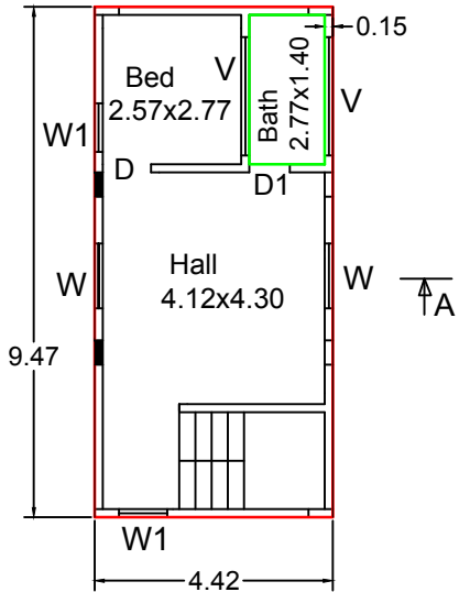
PLAN - First Floor
