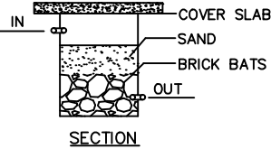
RAINWATER HARVEST
