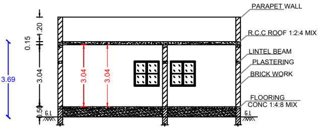
SECTION : "A-B"
