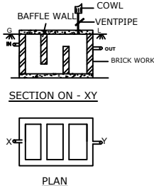
SEPTICTANK DETAILS
