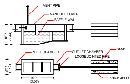
SEPTIC TANK (NOT TO SCALE)
