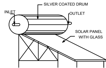
SOLAR SYSTEM NOT TO SCALE
