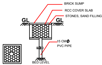
RAIN WATER HARVESTING TANK NOT TO SCALE
