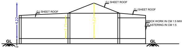
SECTION ON 'XX'
