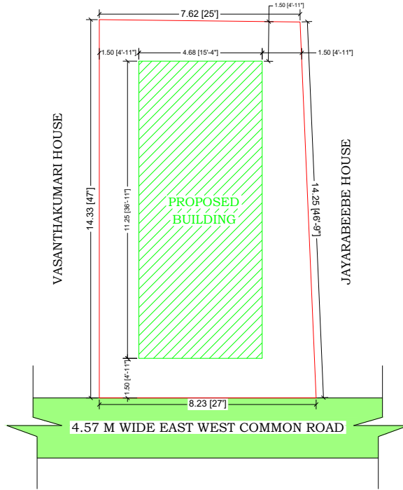
SITE PLAN (SCALE -1:250)
