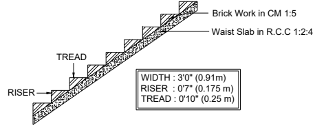
STAIRCASE DETAILS
