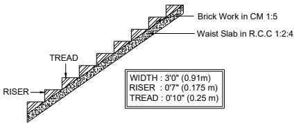
STAIRCASE DETAILS
