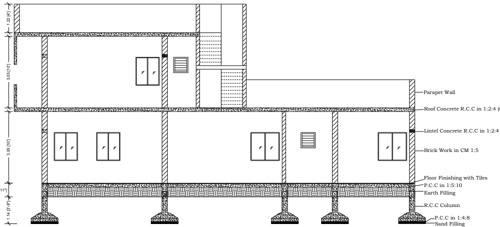
SECTION X-X
