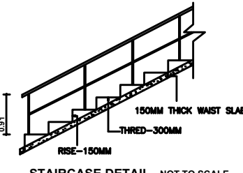
STAIRCASE DETAIL NOT TO SCALE
