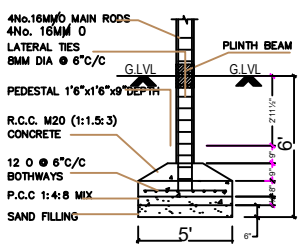
FOUNDATION DETAIL
