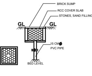
RAIN WATER HARVESTING TANK NOT TO SCALE
