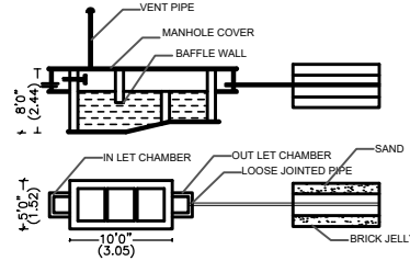
SEPTIC TANK (NOT TO SCALE)
