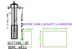
SECTION OF BORE WELL
