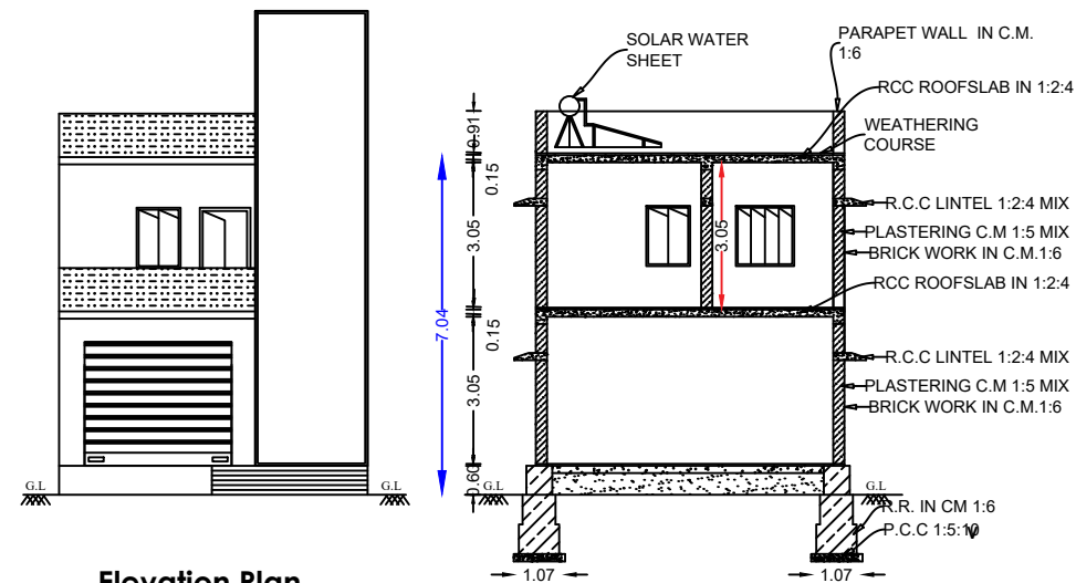
Elevation Plan
