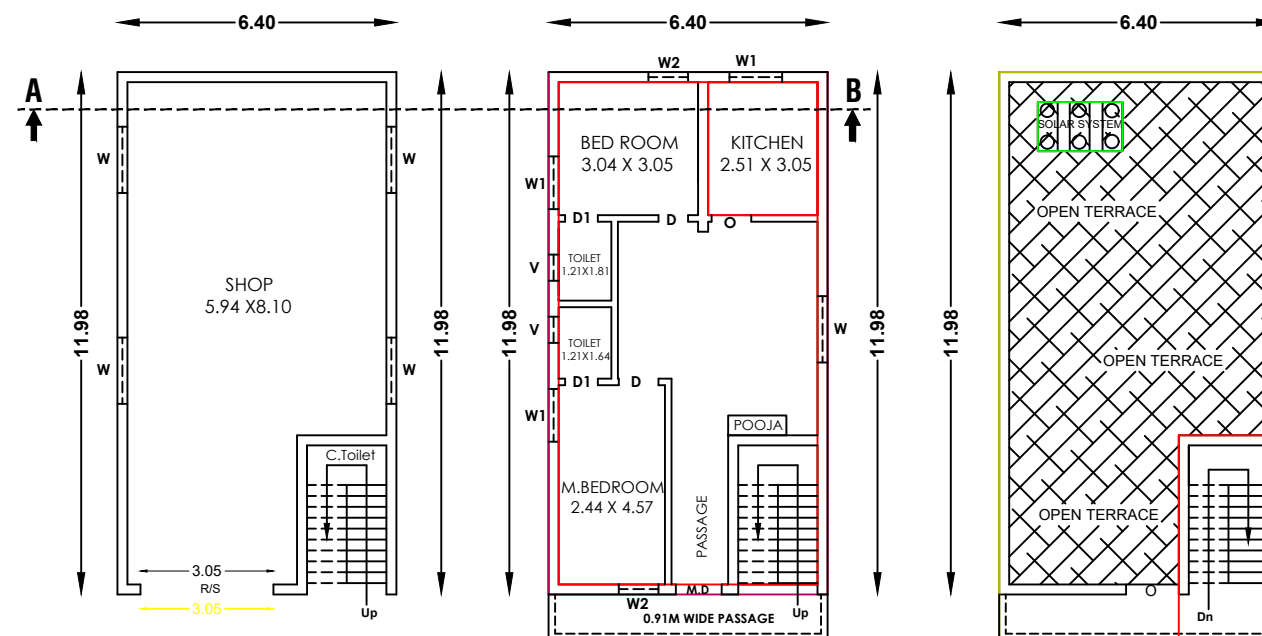
Ground Floor Commercial Plan
