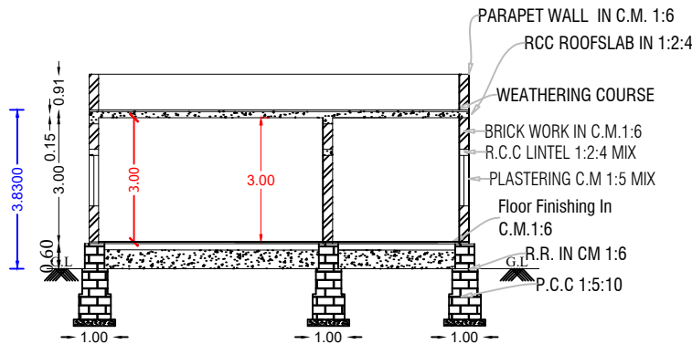
SECTION ON-"AB"
