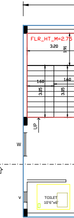
PROPOSED GROUND FLOOR PLAN
