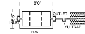
SEPTIC TANK AND DISPERSION TRENCH DETAILS
