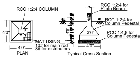
FOOTING DETAILS
