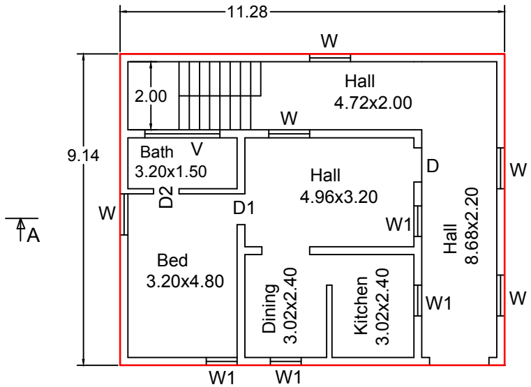
PLAN - Ground Floor
