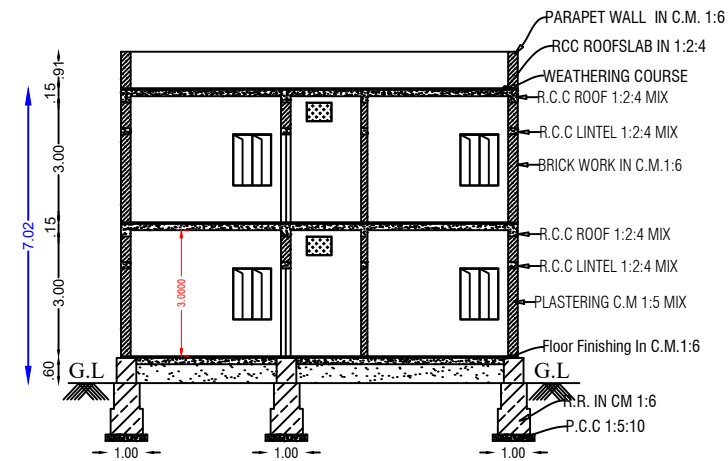
SECTION On-"AB"
