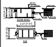
SEPTIC TANK
