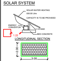
SOLAR SYSTEM
