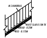
STAIR CASE DETAILS
