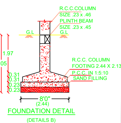
FOUNDATION DETAIL (DETAILS B)
