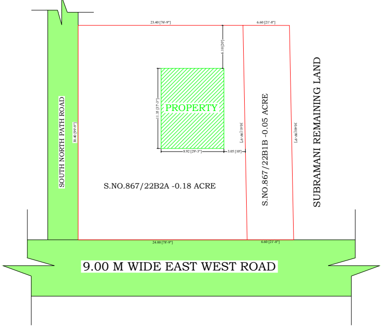
SITE PLAN (SCALE - 1:250)
