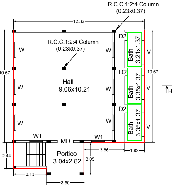
PLAN - Ground Floor (Block - 2)
