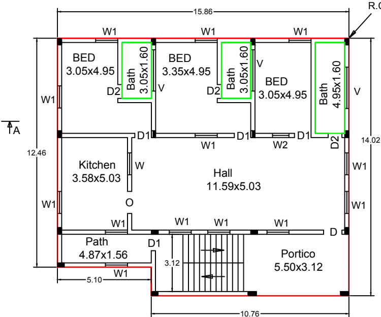
PLAN - Ground Floor (Block-1)
