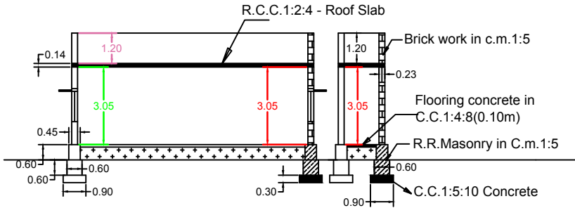
SECTION ON -"BB"
