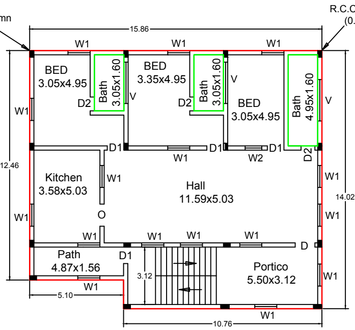
PLAN - First Floor(Block-1)
