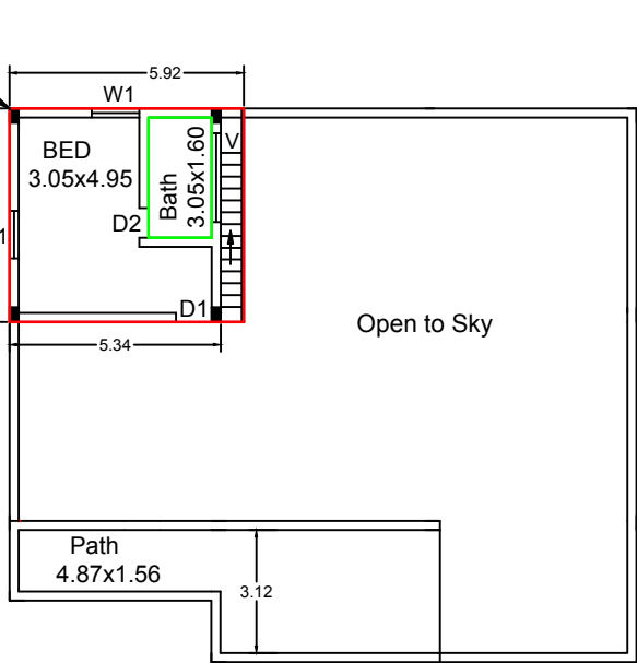
PLAN - Second Floor(Block-1)
