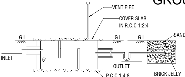
SECTION-AB
