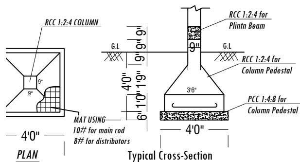
FOOTING DETAILS
