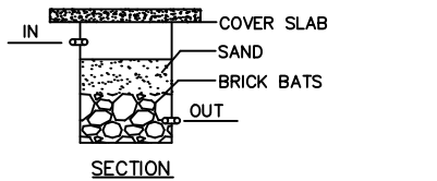
RAINWATER HARVEST
