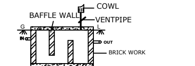
SECTION ON - XY
