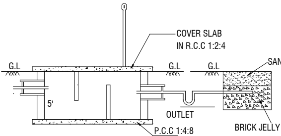
SECTION-AB
