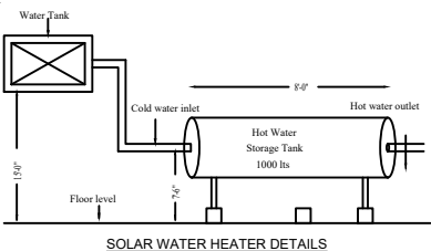
SOLAR WATER HEATER DETAILS
