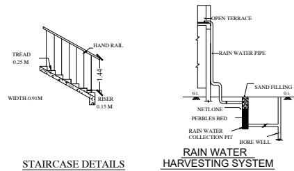
STAIRCASE DETAILS
