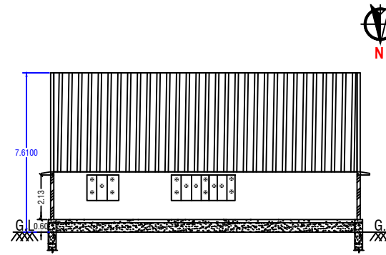
SECTION ON-"AB"
